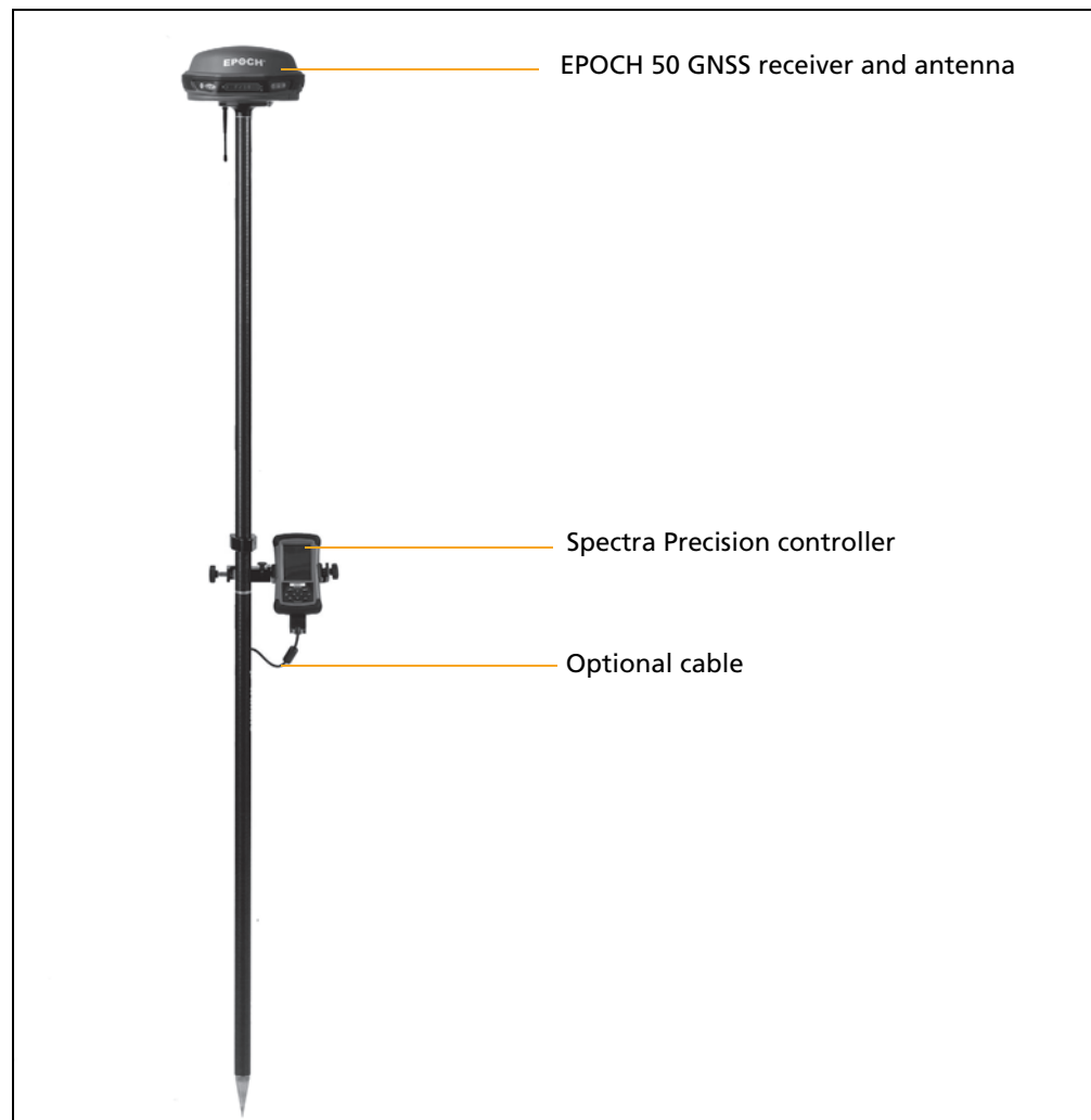
Figure 2.3 EPOCH 50 GNSS receiver set up as a rover receiver
