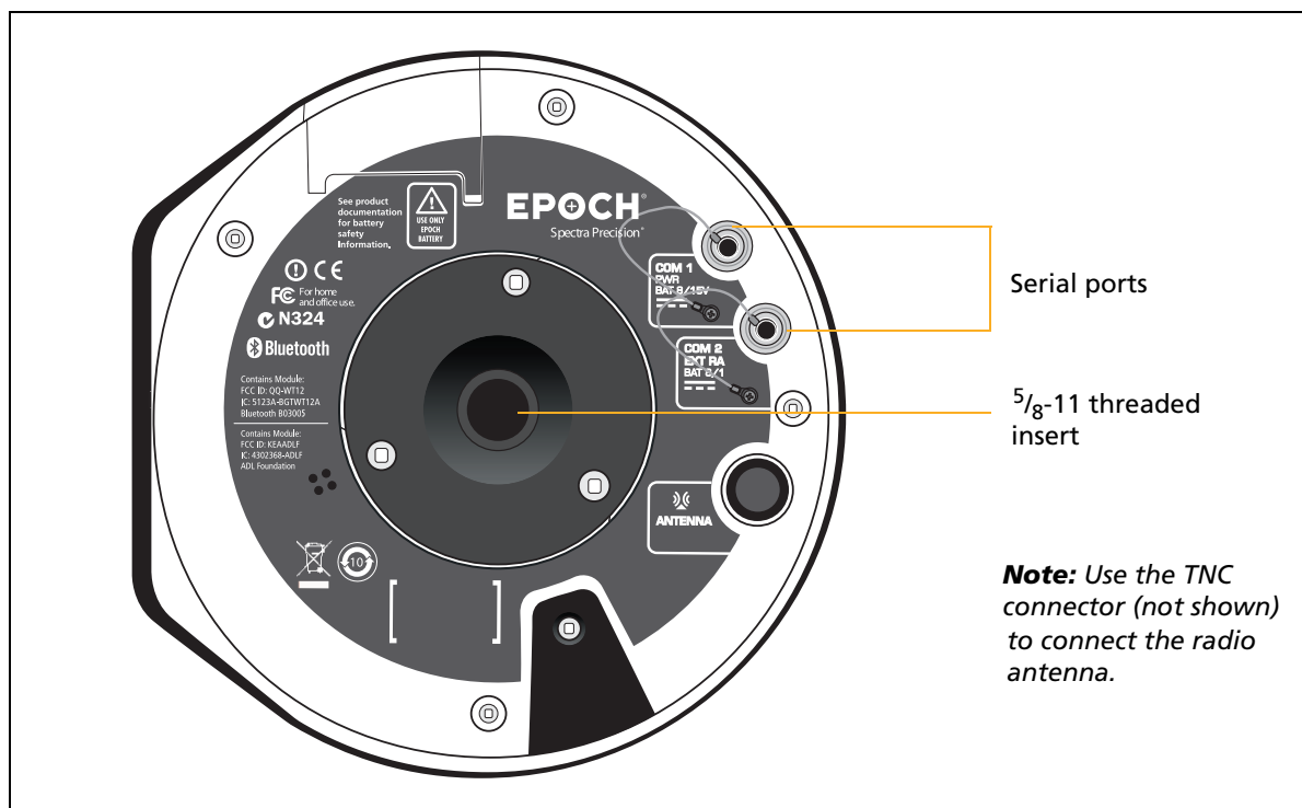
Figure 2.1 Ports and connectors on the receiver
